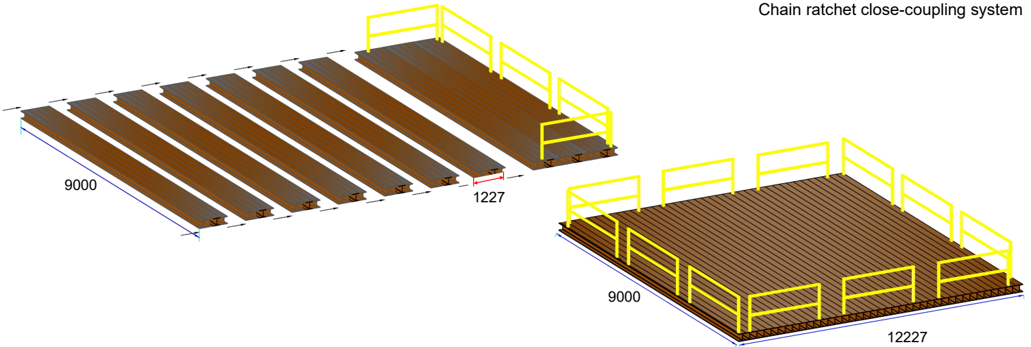
Chain ratchet close-coupling system
